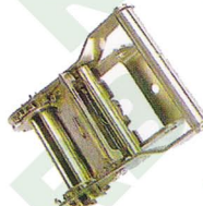
R1058 2" Wide Handle B/S: 1,500Kgs/ 3,300Lbs
