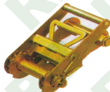
R1060 3" Short Handle B/S: 9,500Kgs/ 20,900Lbs
