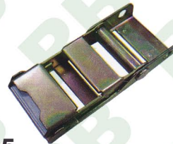
OB035 2" Overcenter Buckle, 50mm, Steel B/S: 2000Kgs/ 4400Lbs
