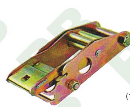
OB036 1 3/4" Overcenter Buckle - One Piece Type, 45mm B/S: 2300Kgs/ 5000Lbs
