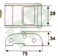
CB010 1" Cambuckle, w/floating Cam, 25mm, B.S.: 800Kgs/ 1760Lbs
