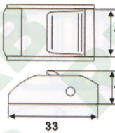
CB006 1 1/2" Cambuckle, 35mm B.S.: 700Kgs/ 1540Lbs
