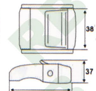
CB007 1 1/2" Cambuckle, 35mm B.S.: 770Kgs/ 1700Lbs
