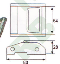
CB013 2" Cambuckle, 50mm, w/Cam B.S.: 1200Kgs/ 2400Lbs
